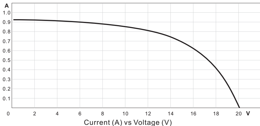
Ampere-Voltage performance of 10W module (GPP0100C140V01)
