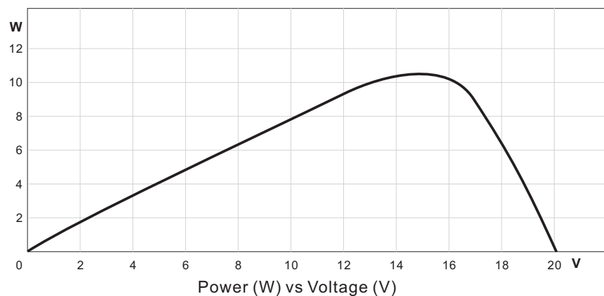
Power-Voltage performance of 10W module (GPP0100C140V01)
