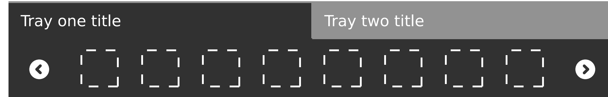
Stacked
