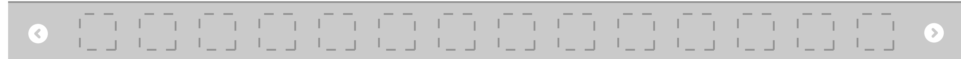
With title
