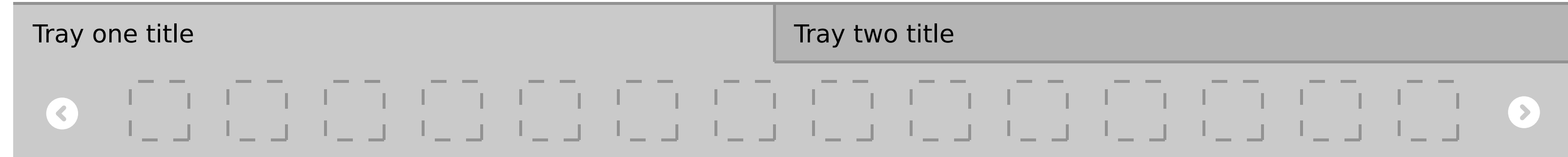
Stacked
