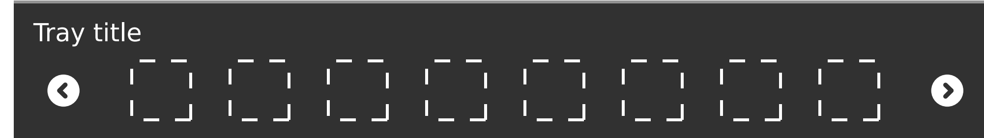
With tabs
