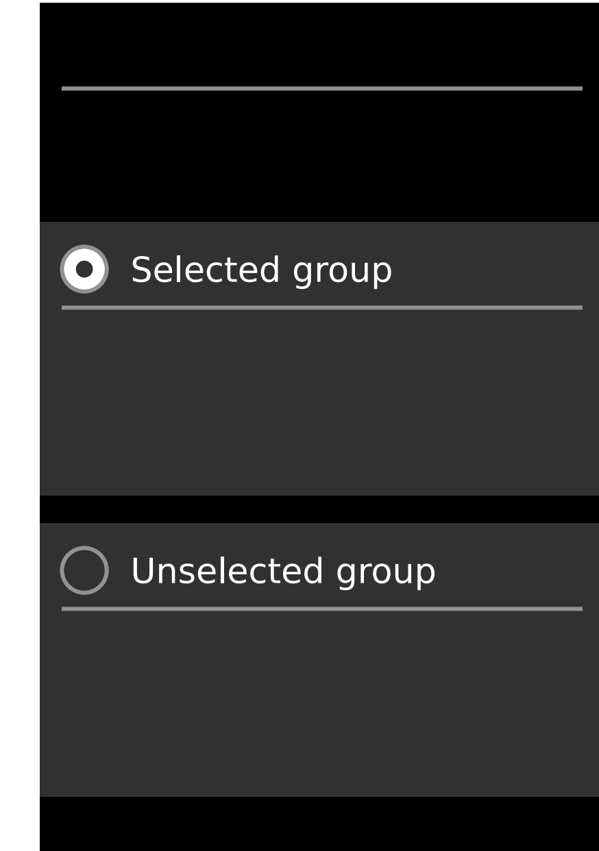
Radio Button
