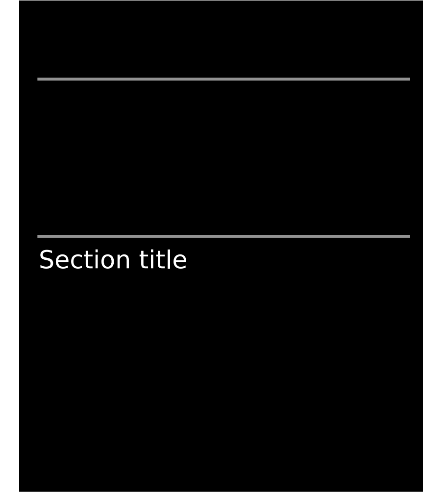
With titles
