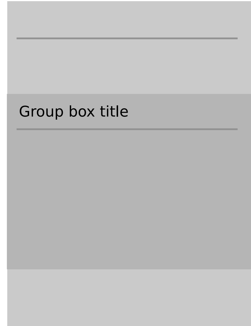
Standard, title
